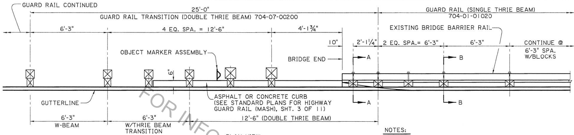
PLAN VIEW
